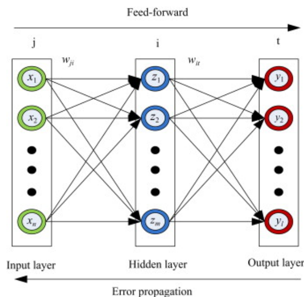
Figure 4. Feed Forward Back propagation Neural Network
