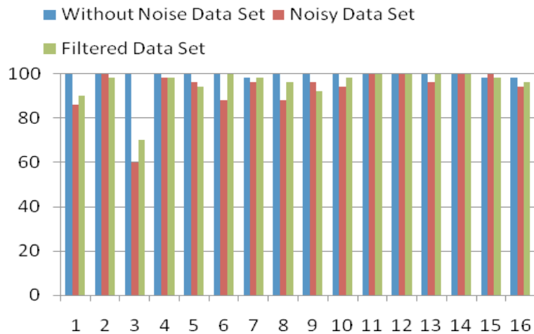
Figure 9. Performance in 2 nd Approach for three data set
