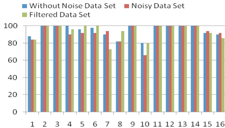
Figure 8. Performance in 1 st Approach for three data set
