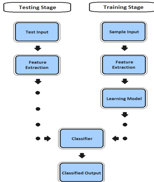
Figure 4. Principal stages of image classification system
