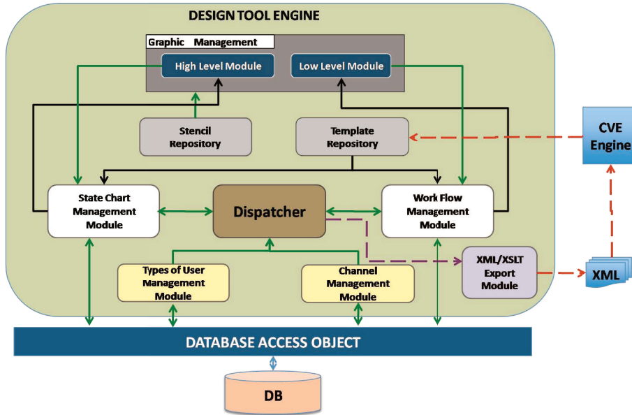
Figure 2: The design tool architecture
