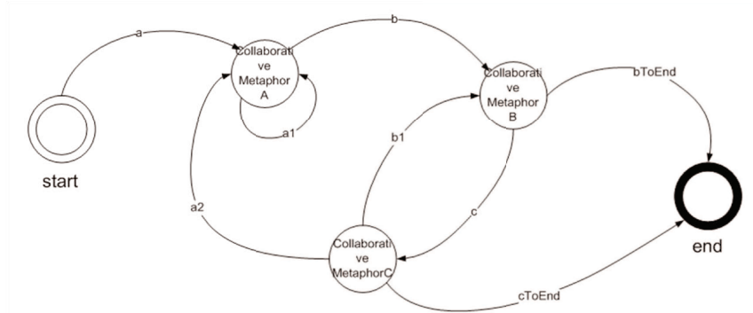
Figure 1: High Level View Example
