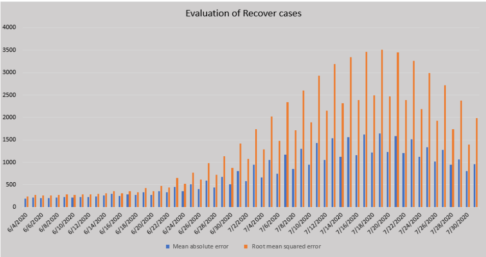
Figure 7: Evaluation of Recover cases
