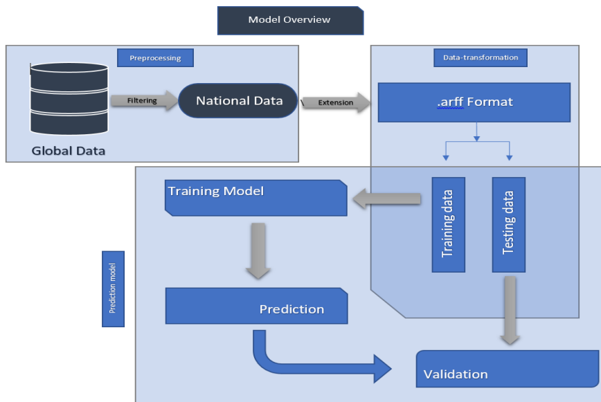
Figure 2: A detail overview of Proposed Methodology
