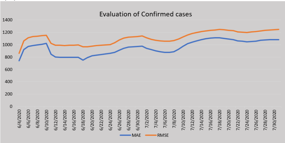
Figure 6: Evaluation of Confirmed cases
