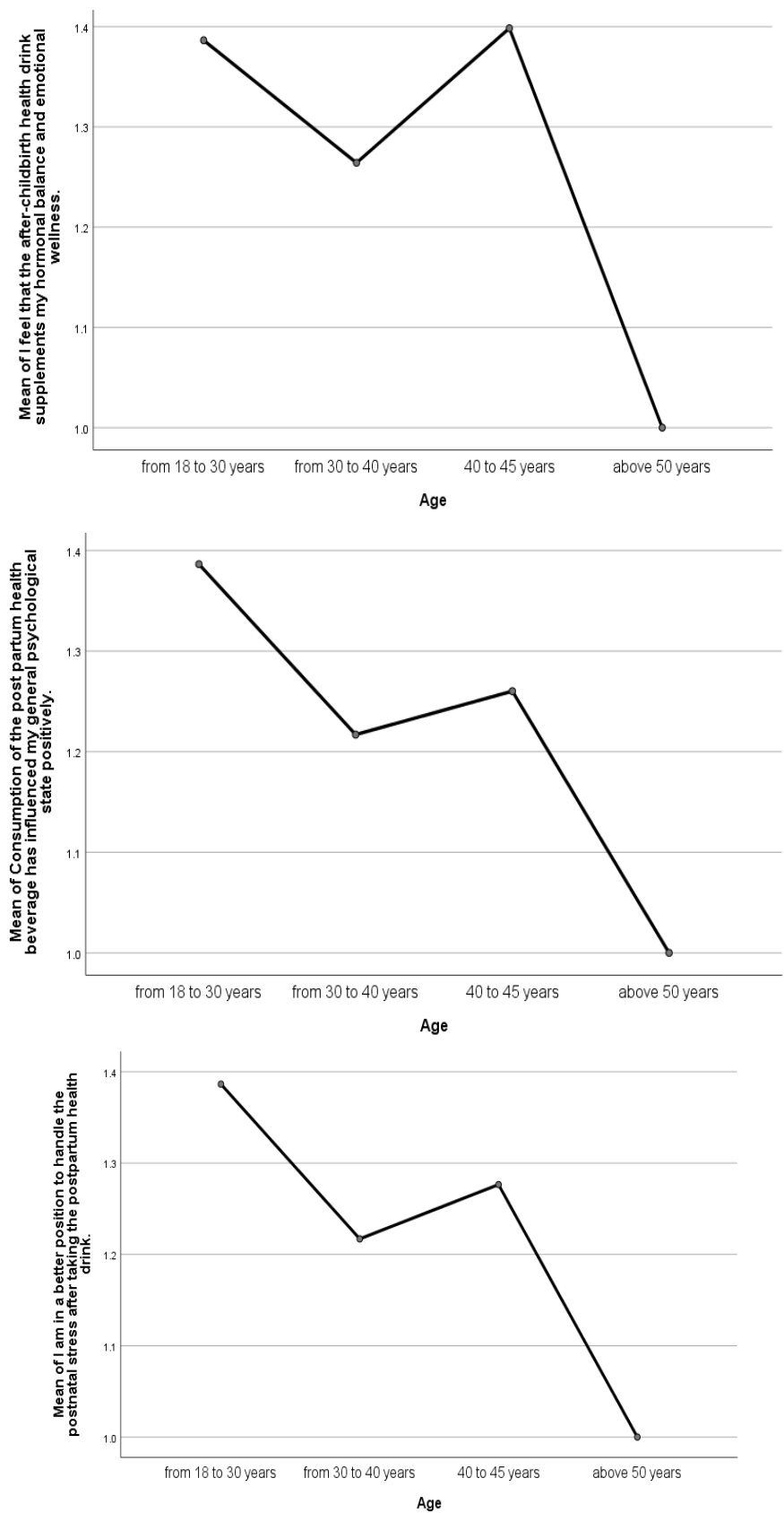
Figure 10. Graphical representation of H3 ANOVA
