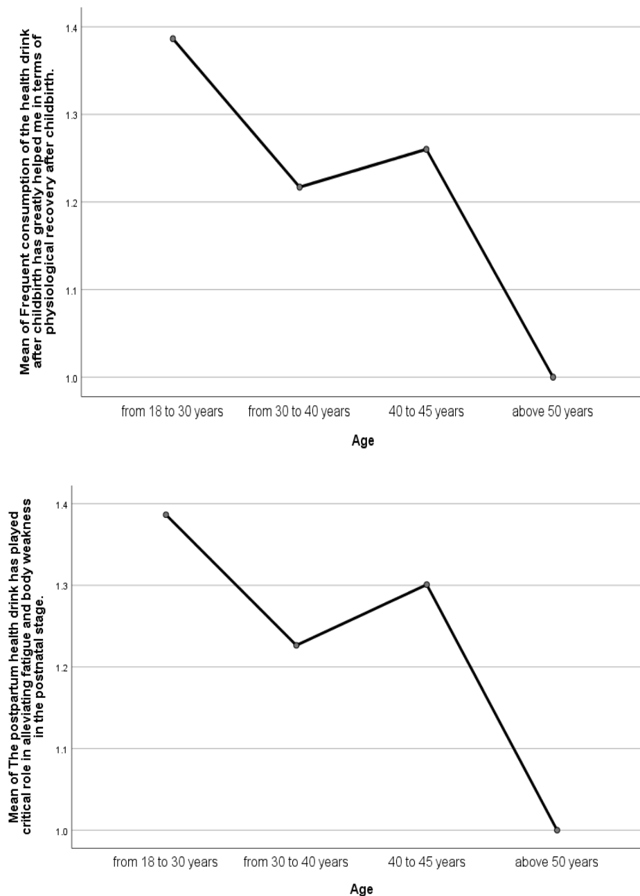
Figure 8. Graphical representation of H1 ANOVA
