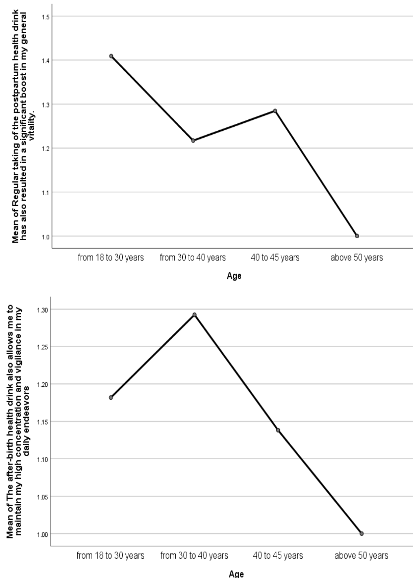
Figure 9. Graphical representation of H2 ANOVA
